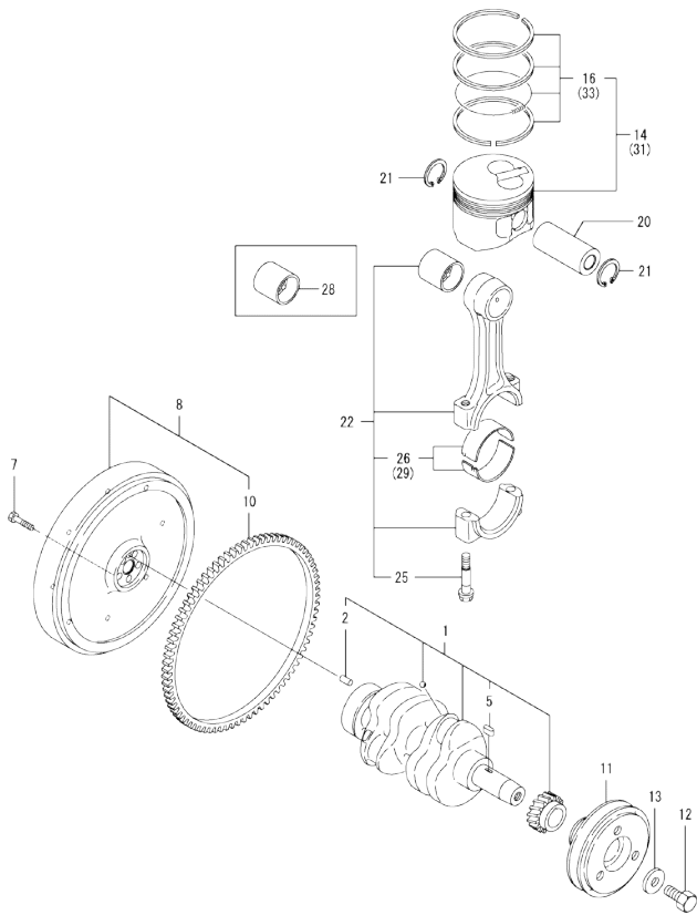
Fig.7. CRANKSHAFT & PISTON
